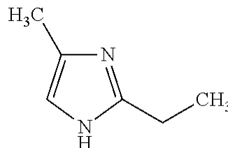
2-ethyl-4-methylimidazole
